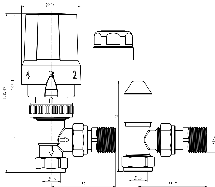
LT-15 Logic 15mm Angled TRV Twin Pack
