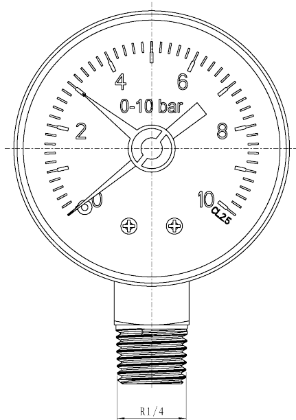
EV-G1014SC Gauge 10 Bar 1/4" Side Connection
